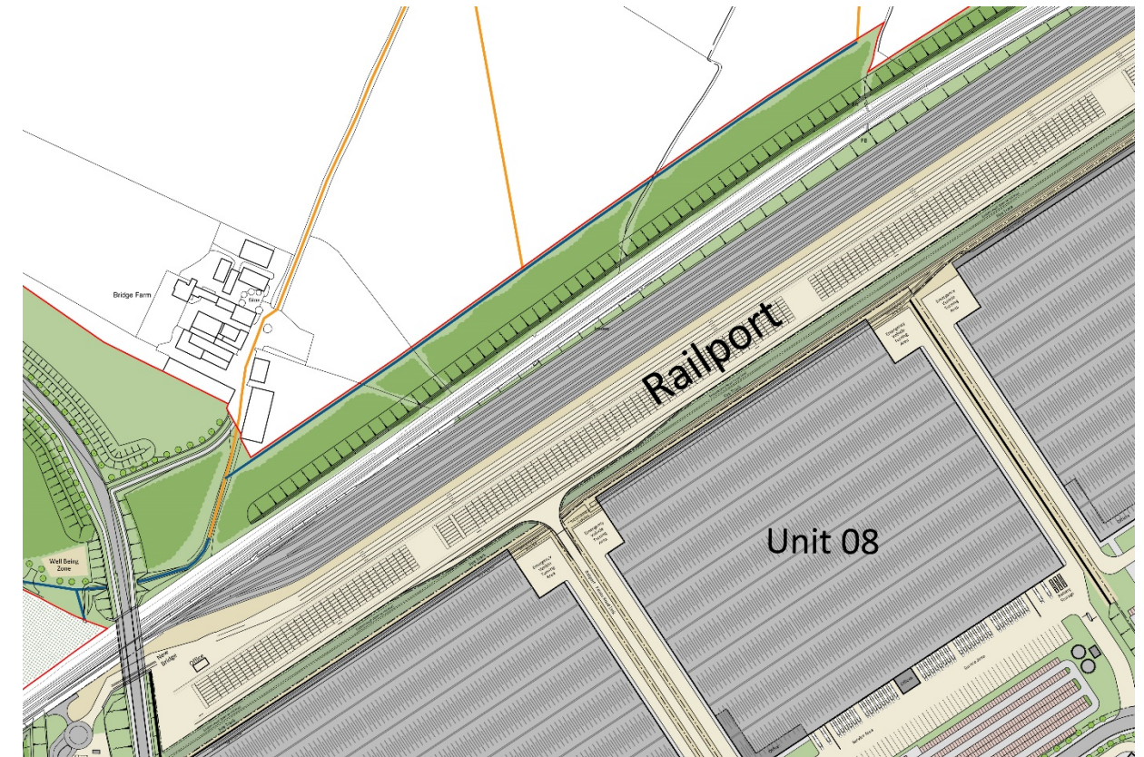
Fig 2739. Extract from illustrative masterplan of Railport.
