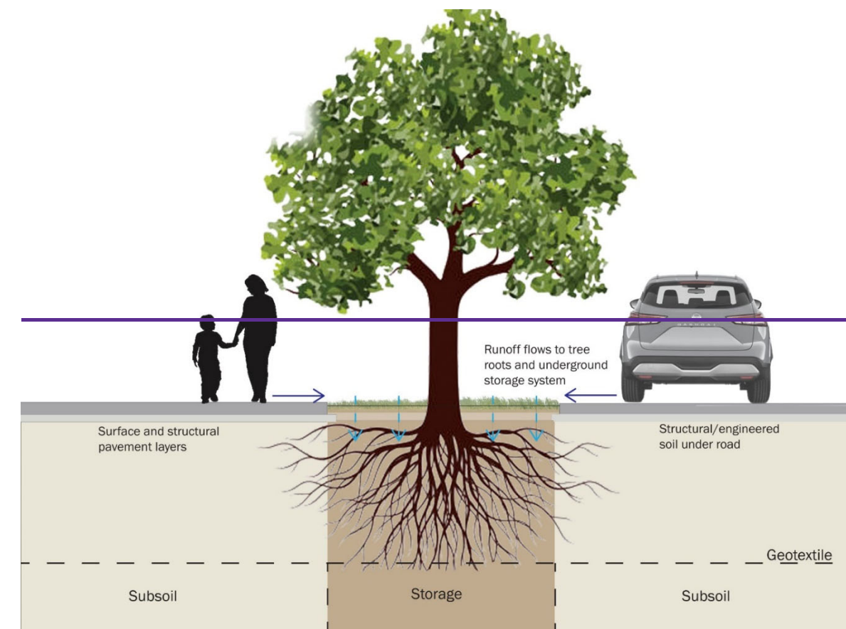
Fig 149. Internal Distributor Road, extract from illustrative landscape strategy plan. Typical Street tree Planting Detail
